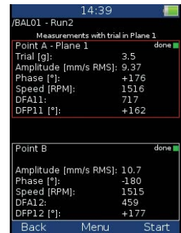
Balancer
