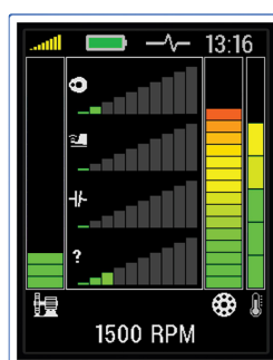
Bearing fault
